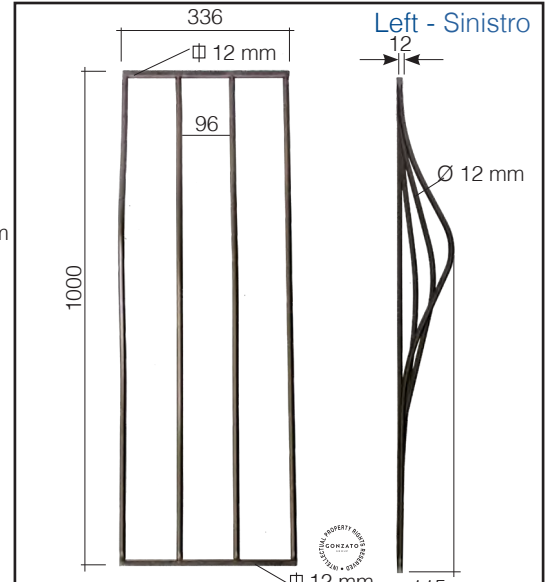
left - sinistro Art. GD294/3 right - destro Art. GD294/3/S Ø 12 mm Ø 12 mm 336 x 1000 mm 336 x 1000 mm
