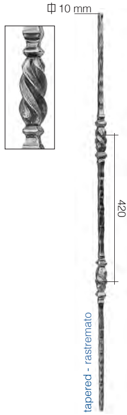
Art. 505/4 Ø 14 x 14 mm H 1000 mm
