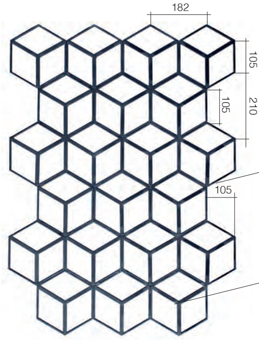
Art. GD287/1 \square 12 \times 6 \text{ mm} + \Phi 12 \text{ mm} 729 x 1000 mm
