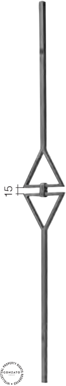
Art. GD181/1 ⌀ 14 mm 130 x 1000 mm
