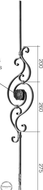
Art. GD271/5 16 x 8 mm 175 x 1000 mm
