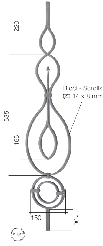
Art. GD177/1 14 mm 205 x 1000 mm
