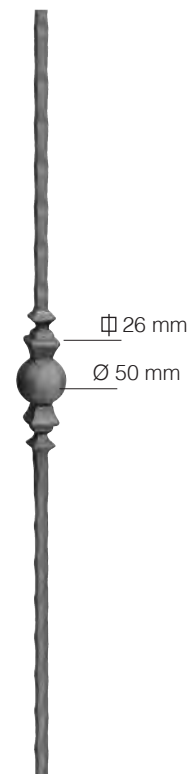
Art. 502/2 14 x 14 mm H 900 mm
