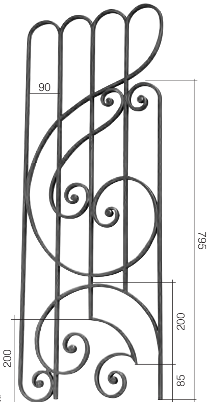
Art. GD225/1 14 x 8 mm 385 x 1000 mm
