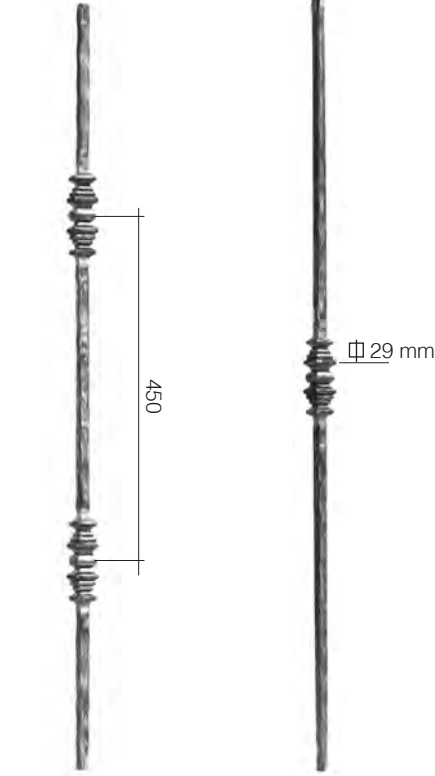
Art. 108/A/1 Ø 12 x 12 mm H 1000 mm
