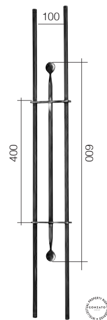
Art. GD67/1 □ 12 mm L 125 mm H 1000 mm
