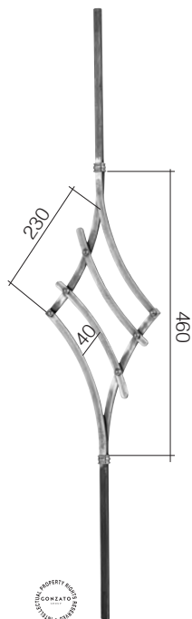
Art. GD20/8 \varnothing 12 mm 200 x 1000 mm
