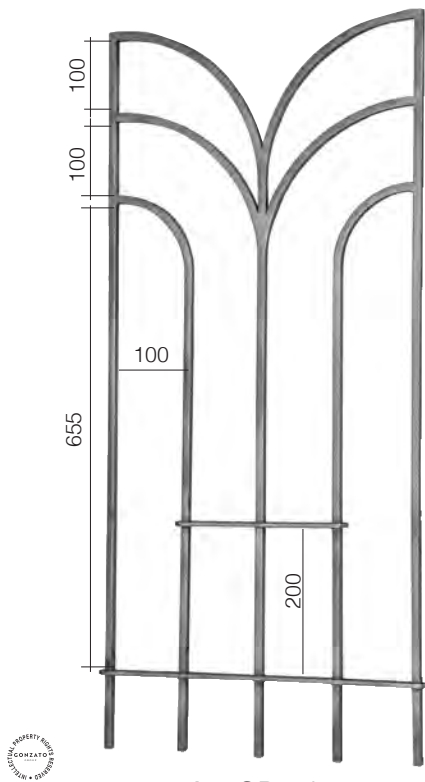
Art. GD68/1 \Phi 12 x 12 mm 480 x 1000 mm
