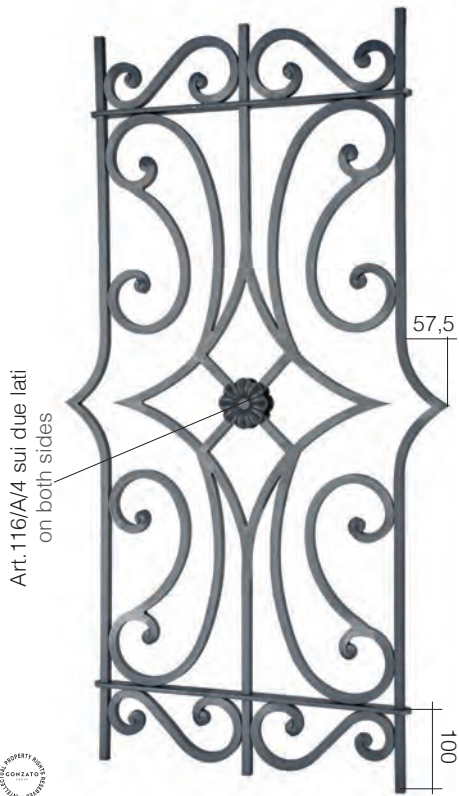
Art. GD61/3 \varnothing 12 mm 515 x 1000 mm
