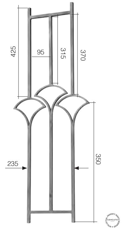
Art. GD186/3 \square 14 mm 390 x 1000 mm
