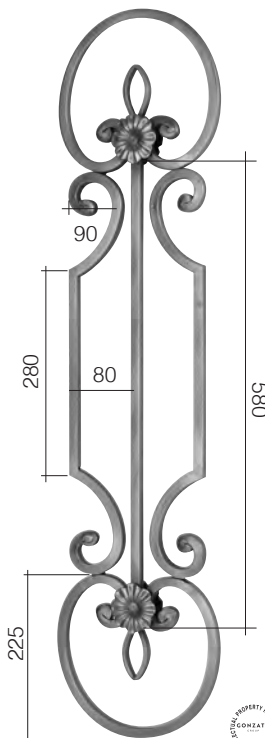
Art. GD31/2 \varnothing 14 x 14 mm 245 x 1000 mm
